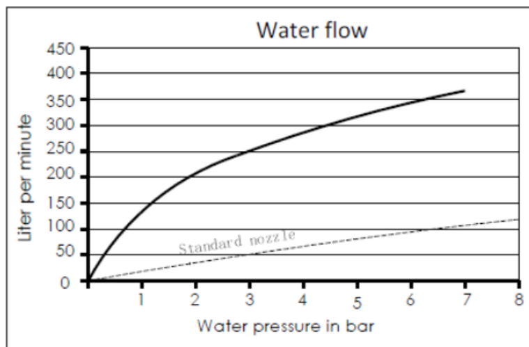
Flow-pressure diagram
