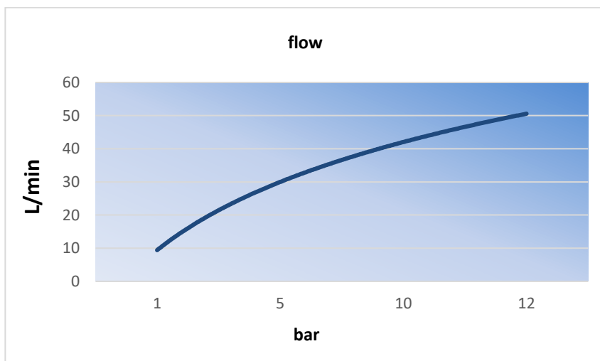
Water flow in l/min when operating lever is fully squeezed, depending on pressure
