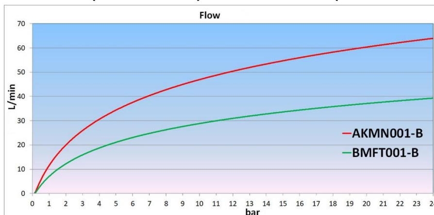
Water flow in l/min when operating lever is fully squeezed, depending on pressure
