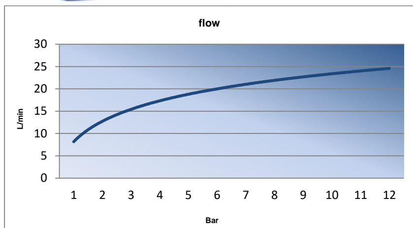
Water flow in l/min when operating lever is fully squeezed, depending on pressure
