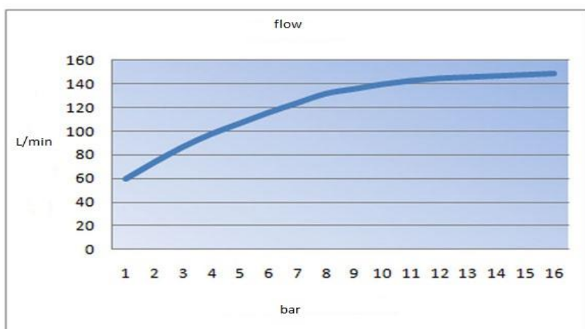
Water flow in L/min at fully opened nozzle, depending on pressure
