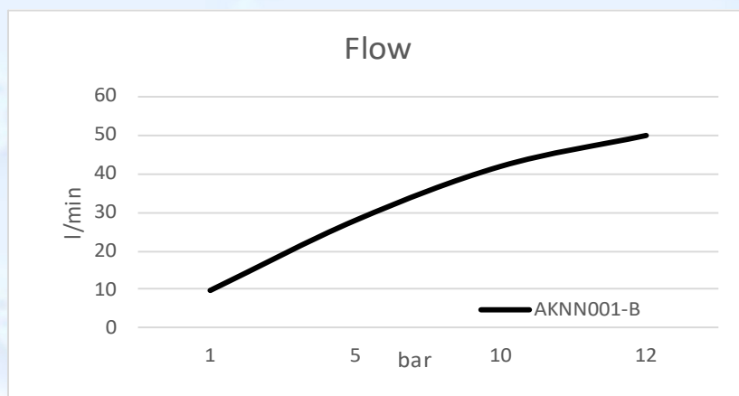
Water flow of the AKNN-series in relation to the pressure
