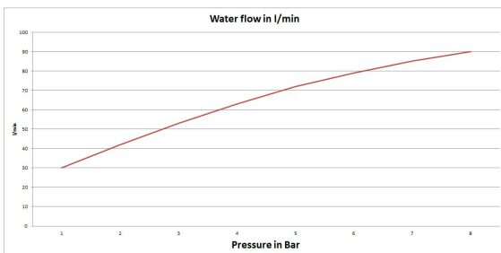
Water flow of the shower head in relation to the pressure.
